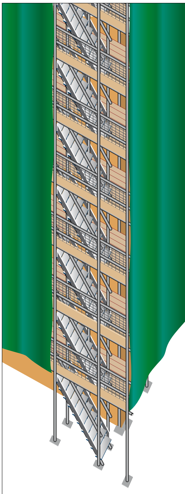
Figure 5 Where sheeted scaffolds form part of the escape route, avoid sheeting the access points so that smoke can escape and the fire service can gain access. Some scaffold components have been omitted for clarity
