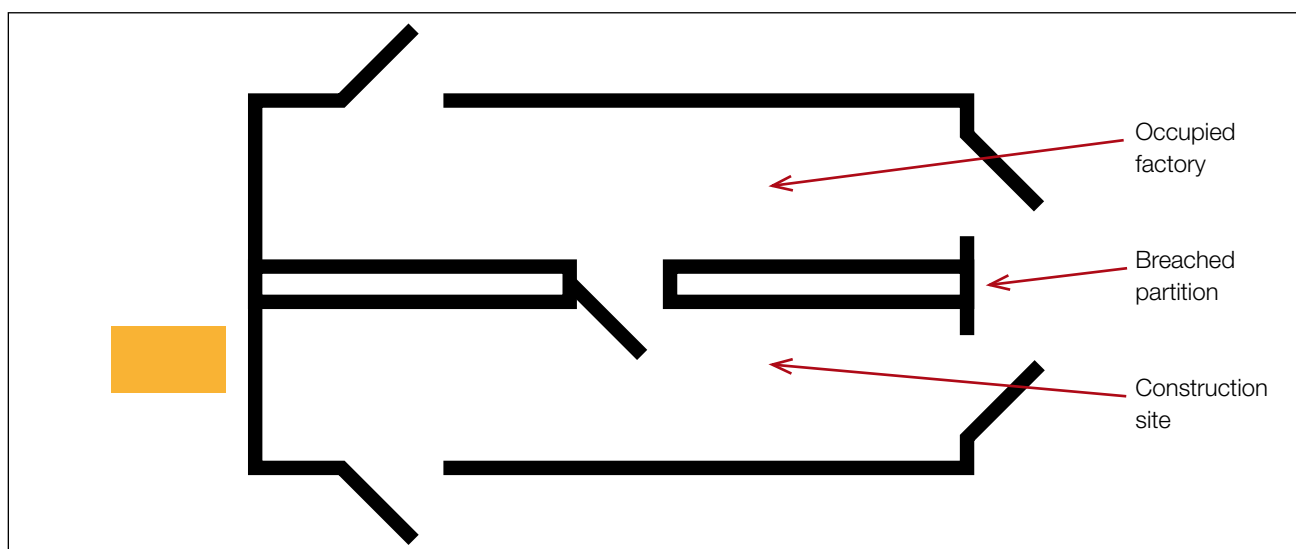
Figure 18 Fire safety requirements for construction sites in shared location/premises with breached partition
