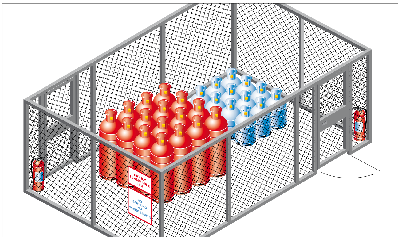
Figure 4 When large amounts of LPG are stored, provide purpose-built, secure accommodation for it
