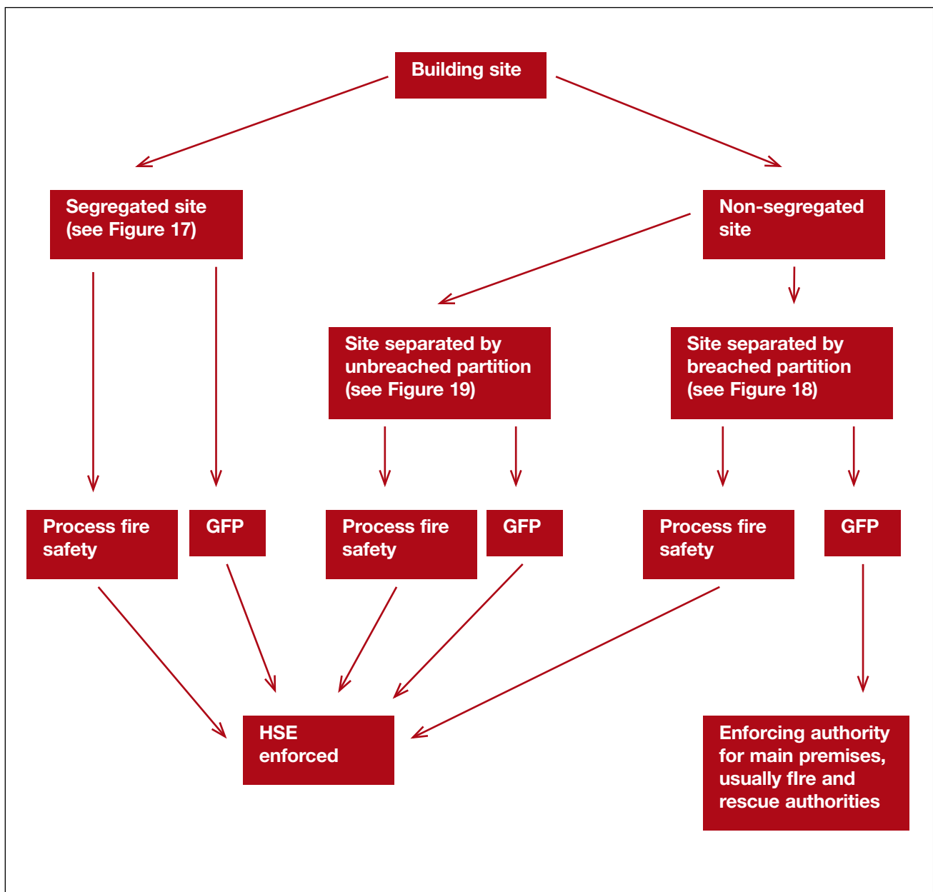
Figure 20 Flow chart to summarise fire safety enforcement on construction sites
