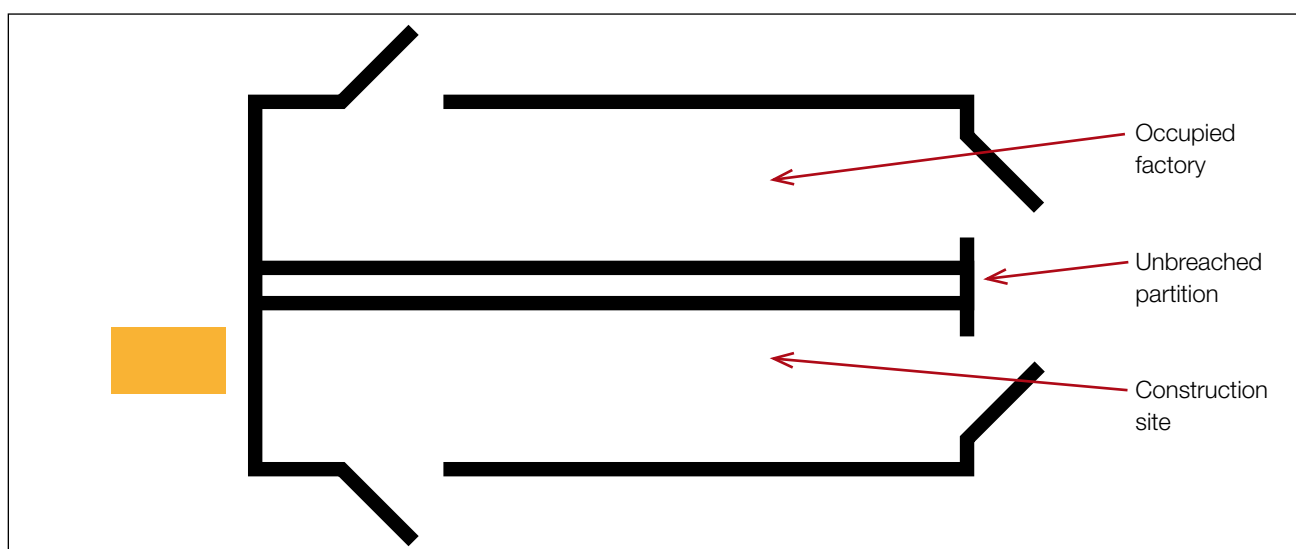
Figure 19 Fire safety requirements for construction sites in shared location/premises with unbreached partition
