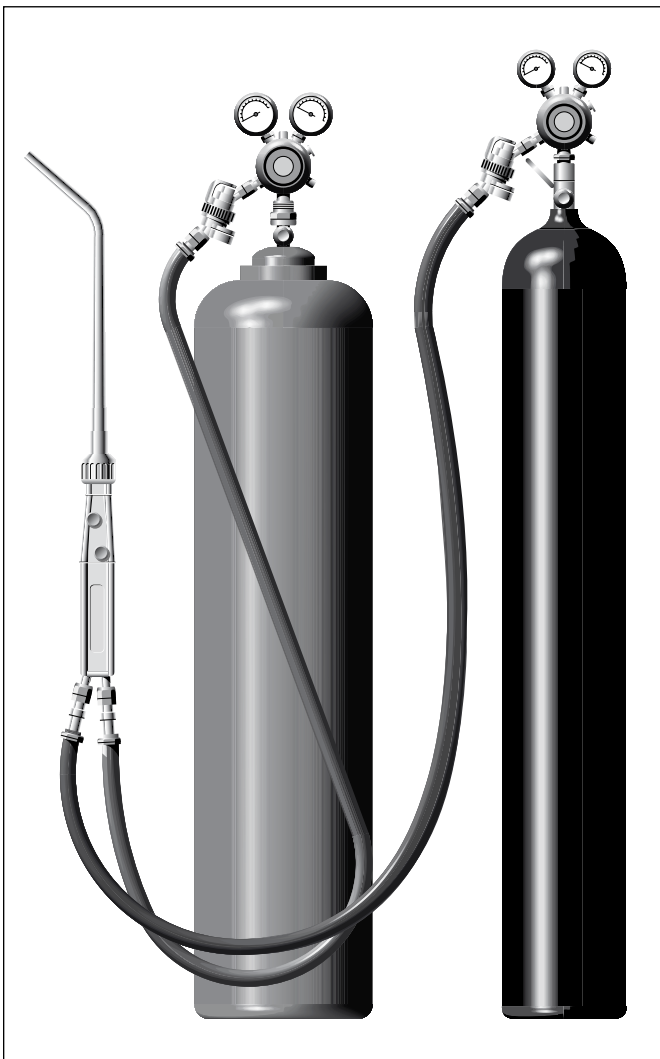
Figure 3 Typical equipment used in gas welding and allied processes. Note: (a) flashback arresters and (b) non-return valves
